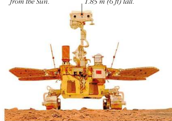
The 7.6 m (25 ft) long solar panels generate power from the Sun.
